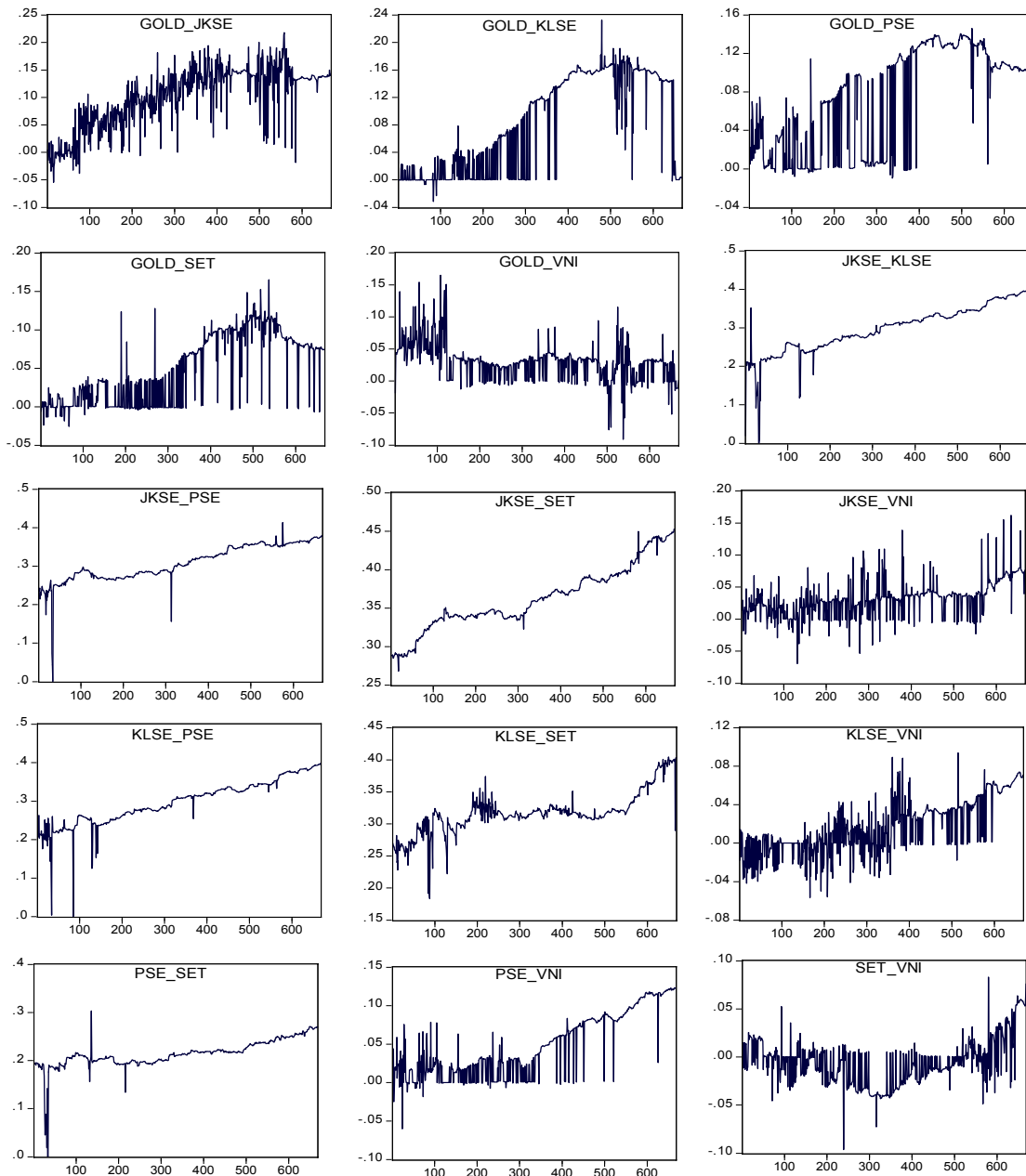
Figure 2: Dynamic paths of pair return conditional correlations based on VARMA-AGARCH (window size=1000 and moving windows=668)
